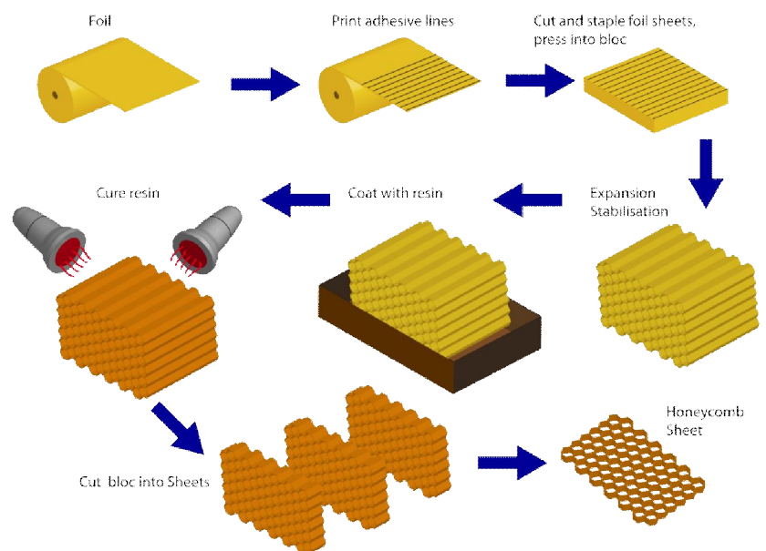
Production process for aramid honeycomb
